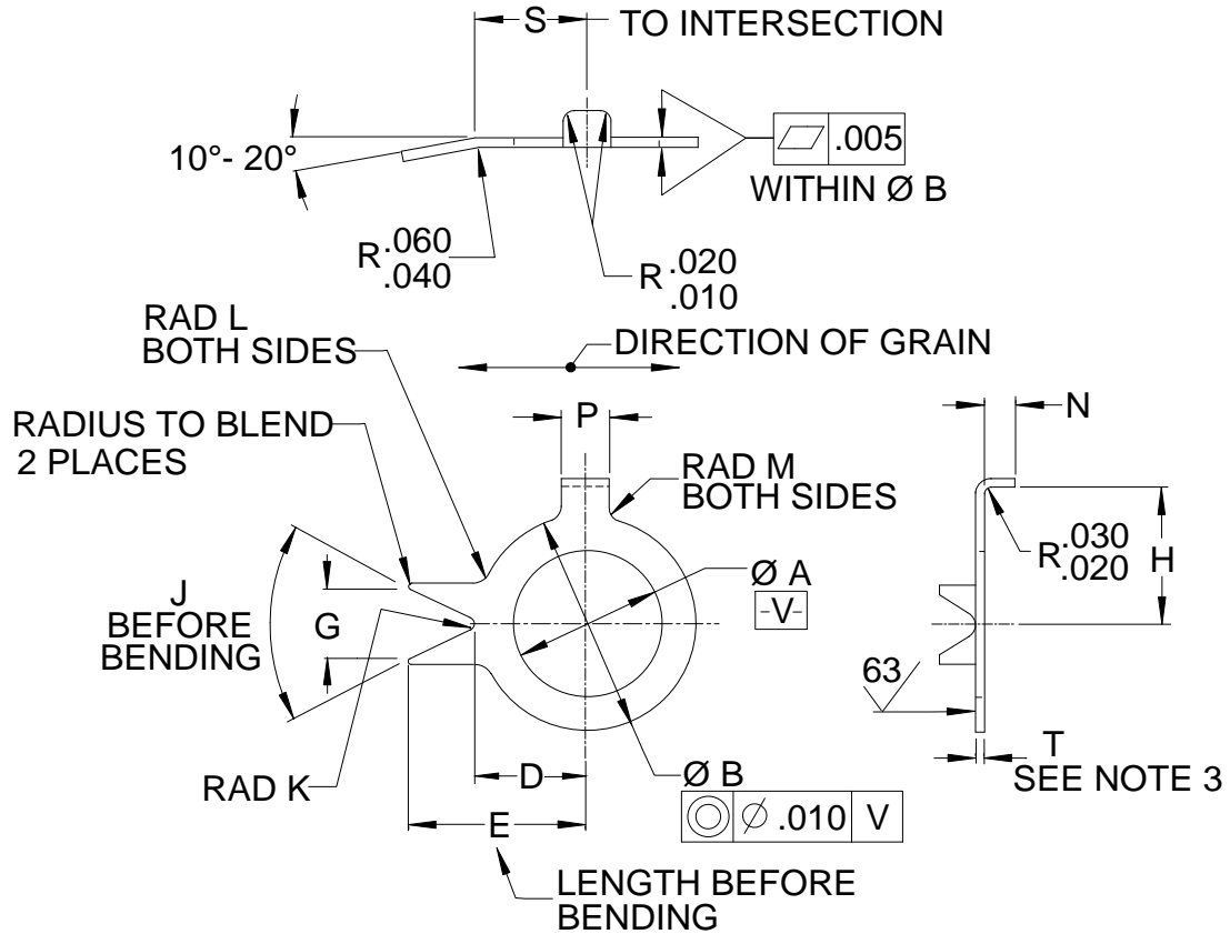
FIGURE 1 - WASHER
